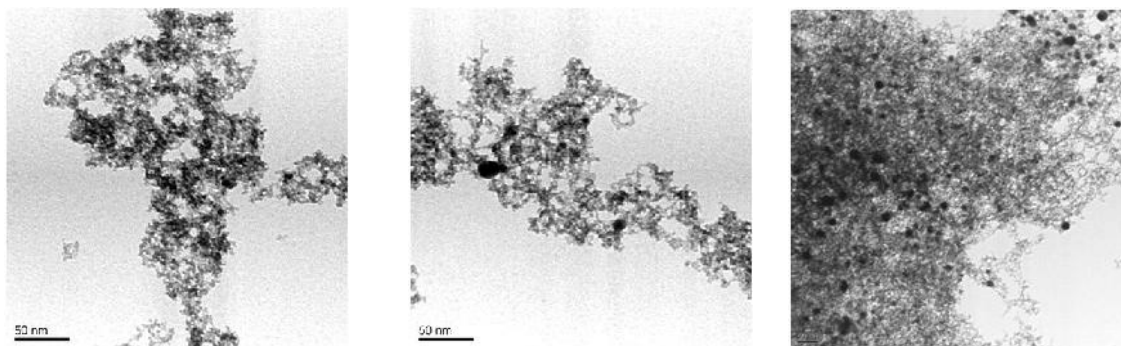
Figure 3.6. Representative TEM images for as prepared samples of 1% Au/CeO 2 , 5% Au/CeO 2 and 5% Au/ZrO 2 from left to right respectively.
