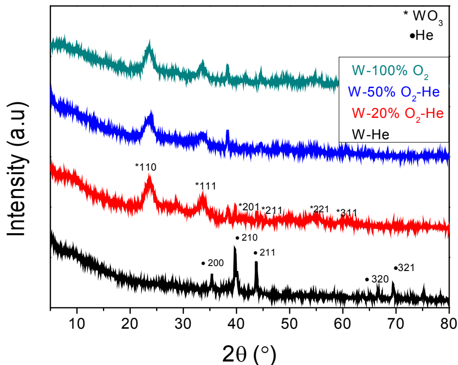
Figure 5.3. X-ray diffraction patterns of tungsten and tungsten oxide nanoparticles prepared by LVCC under He and O 2 /He atmospheres.
