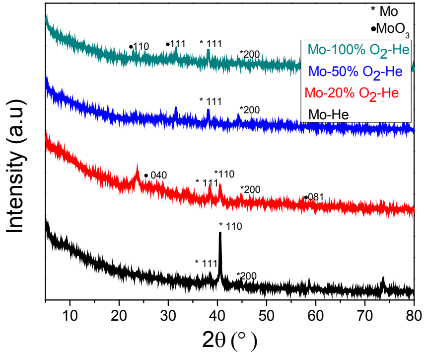
Figure 5.2. X-ray diffraction patterns of molybdenum and molybdenum oxide nanoparticles prepared under pure He and \text{O}_2/\text{He} atmospheres using LVCC.
