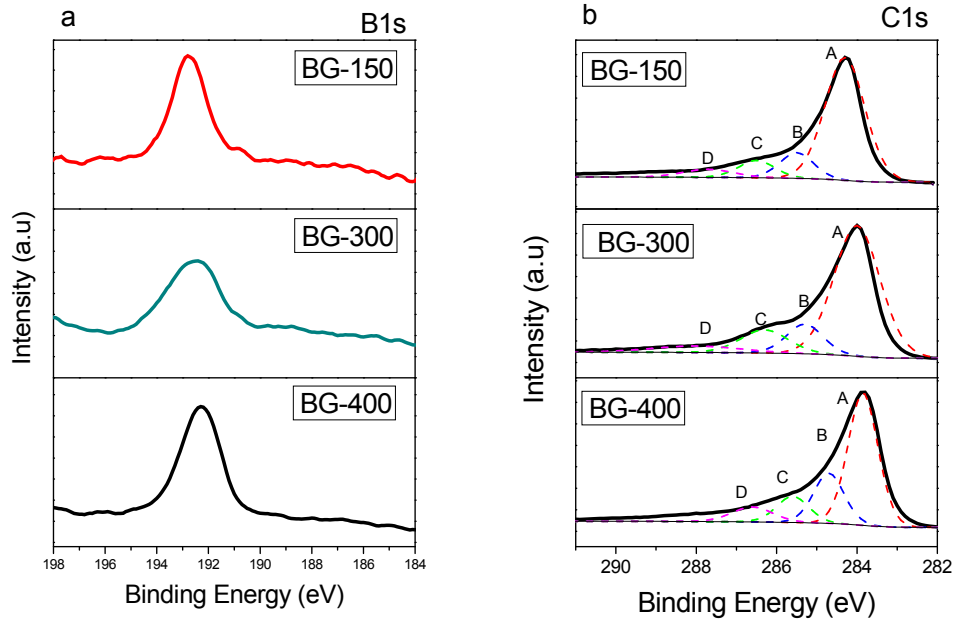
Figure 4.17. XPS spectra of (a) B1s and (b) C1s of boron doped graphene (BG) samples prepared by LVCC under different partial pressure of B_2H_6 gas.
