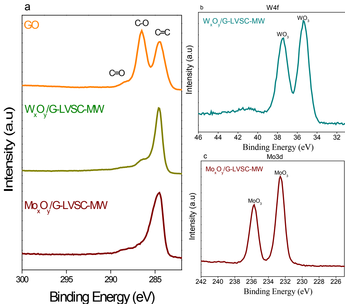
Figure 5.31. (a) C1s XPS spectra for GO, W_xO_y/G and Mo_xO_y/G , (b) W4f XPS spectra for W_xO_y/G and (c) Mo3d XPS spectra for Mo_xO_y/G .
