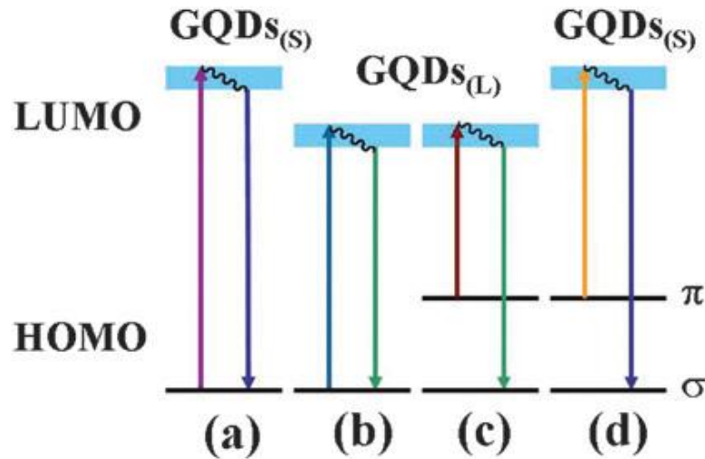
Figure 4.35. A schematic illustration of various typical electronic transitions processes of GQDs. (a and b) Normal PL mechanisms in GQDs for small (S) and large (L) sizes, and (c and d) upconverted PL mechanisms in GQDs for large size and small sizes. 190
