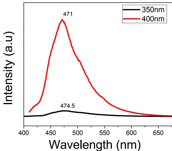
Figure 6.14. Photoluminescence of colloidal suspension of Si nanoparticles capped with acetonitrile at two different excitation wavelengths of 350 nm and 400 nm. Sample was prepared by LVSC.
